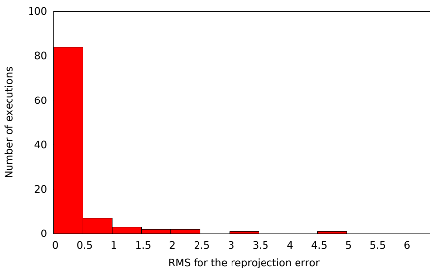
Figure 5.10: Reprojection error distribution. 84 executions obtained an RMS error below 0.5 pixels.
