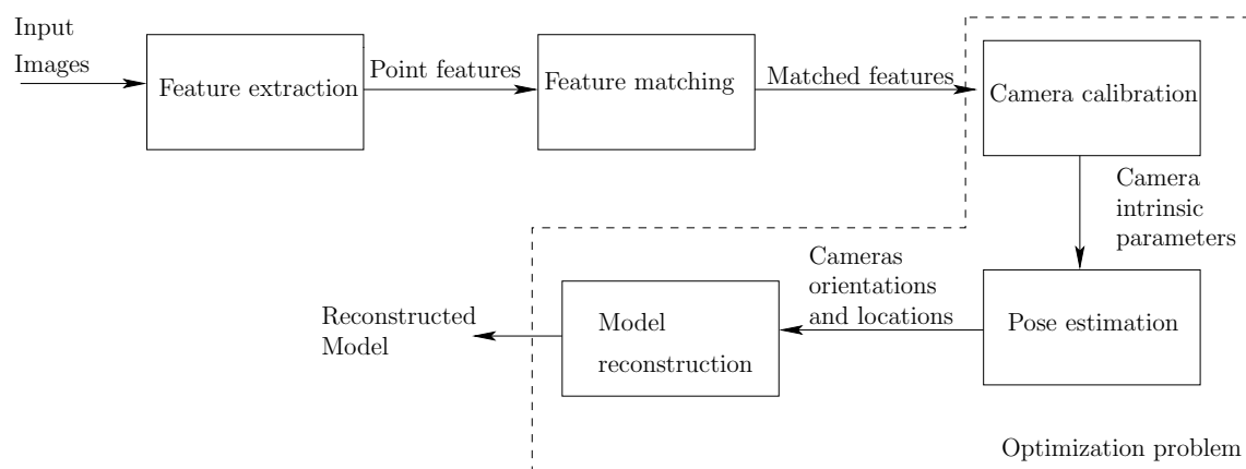
Figure 1.1: First study and the involved subproblems.
